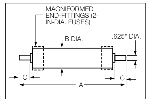
Figure 5. NX clip style dimensional drawing. (See Table 4 for dimensions.)
