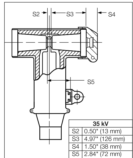
Figure 3. Bol-T Stacking Dimensions.
