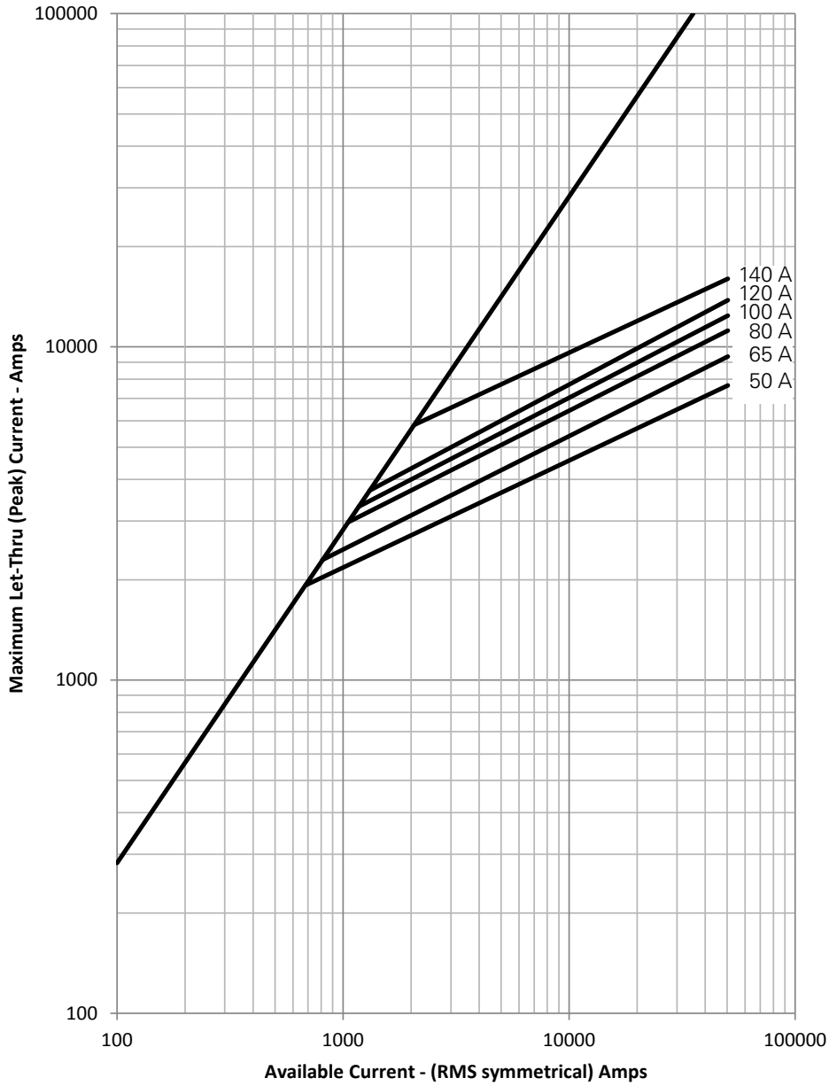
Figure 4. Peak let-through curves for 38 kV ELSP backup current-limiting fuse.
