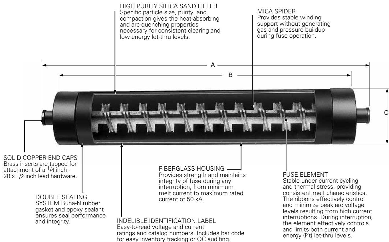
Figure 1. 2" diameter ELSP current-limiting back-up fuse cutaway shows design characteristics.
