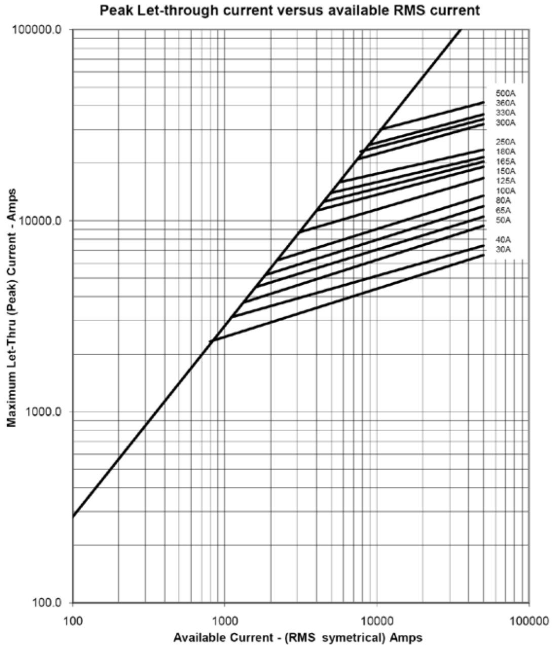
Figure 3. Peak let-through curves for 8.3 kV, 9.9 kV, 15.5 kV, 17.2 kV and 23 kV ELSP backup current-limiting fuse.
