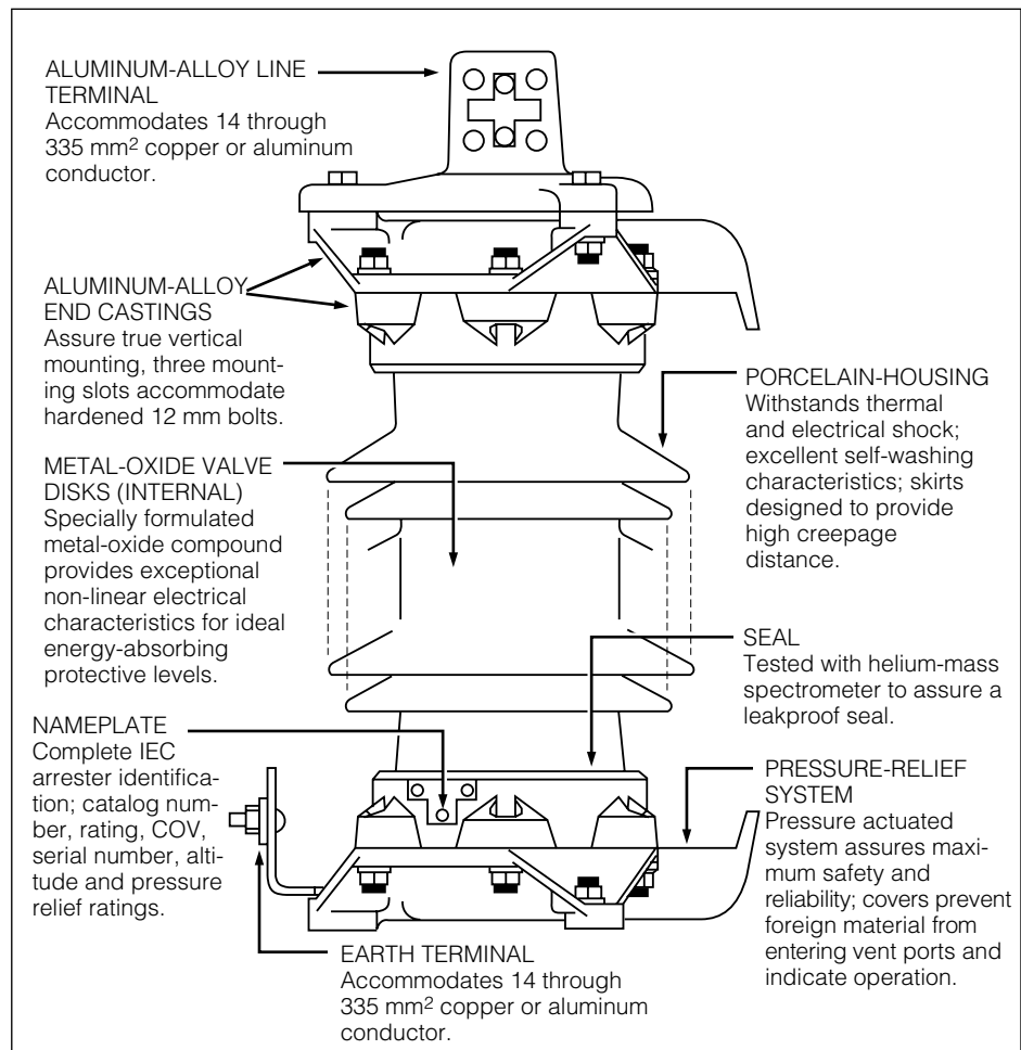
Figure 2. VariSTAR Type AZG2 Arrester Construction Details.
