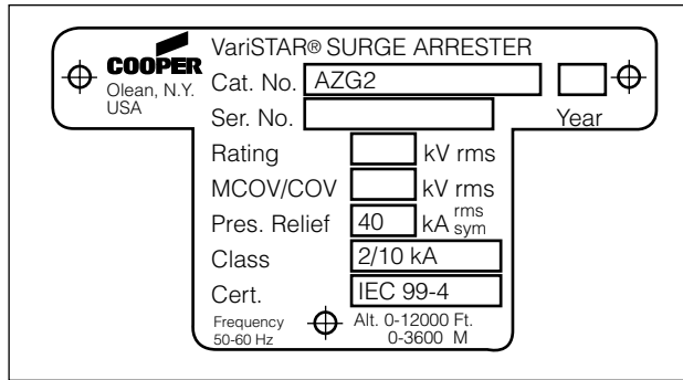
Figure 7. Arrester Nameplate.
