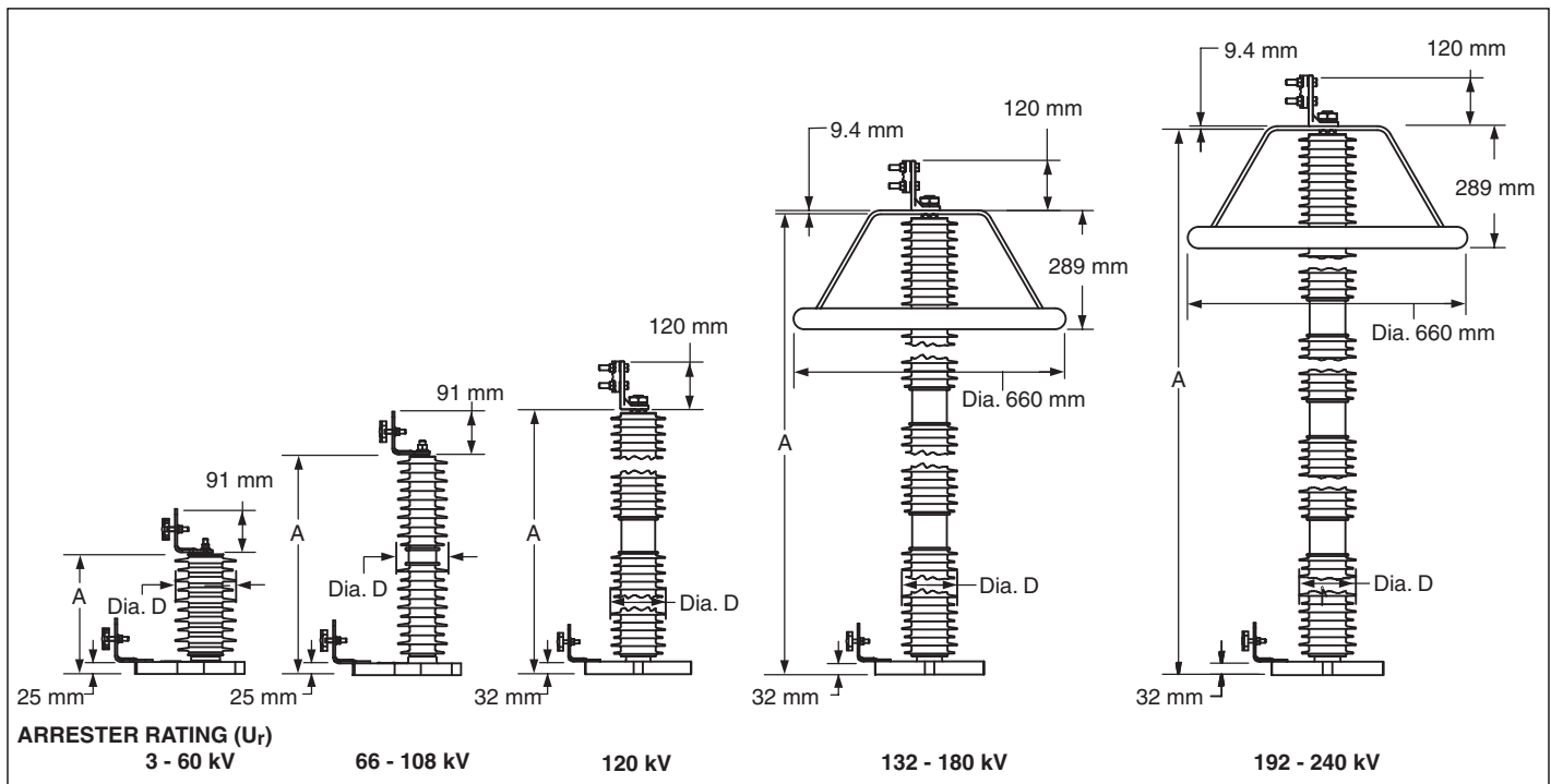
Figure 5. Outline Drawing of Standard UltraSIL Housed VariSTAR Type U2 Surge Arresters.
