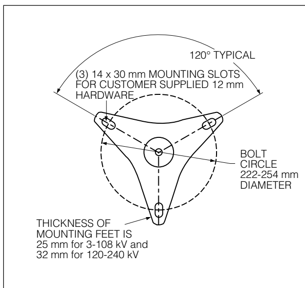
Figure 8. Base mounting.
