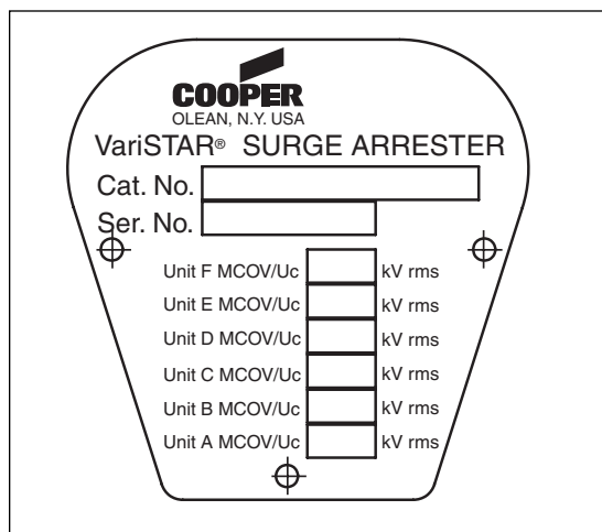
Figure 7. Detail of unit nameplate on arrester base.
