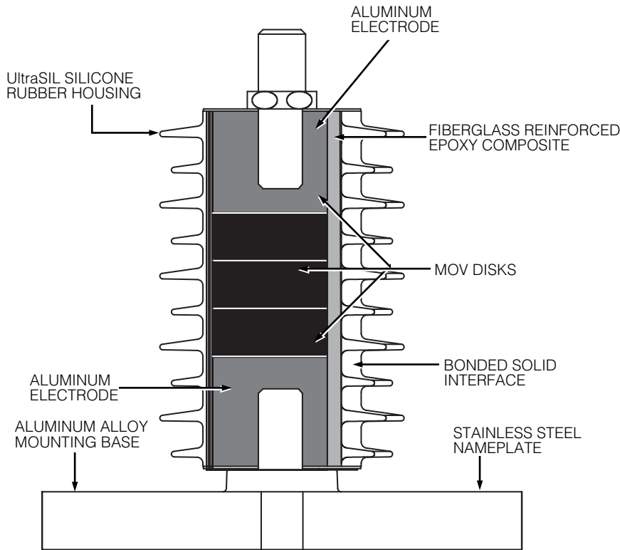
Figure 2. Cutaway illustration of UltraSIL Housed VariSTAR Class 2 Arrester.
