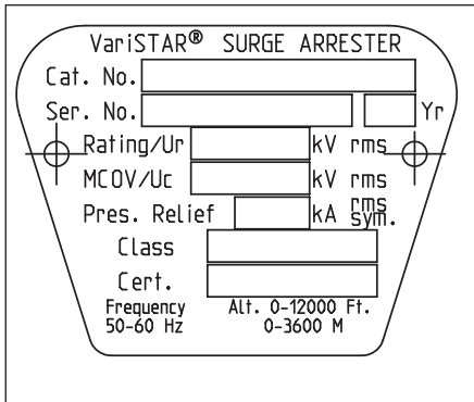
Figure 6. Arrester base nameplate (English version).
