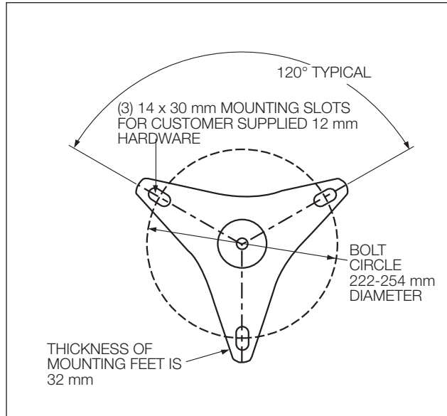
Figure 8. Base mounting.
