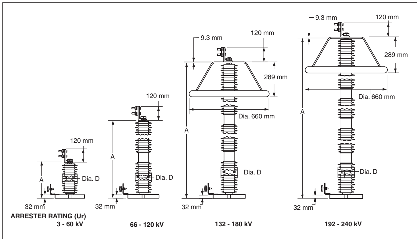
Figure 5. Outline drawing of Standard UltraSIL Polymer-Housed VariSTAR Type U4 Arresters.
