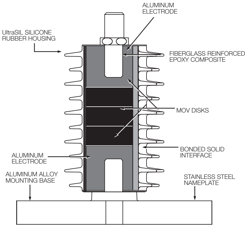
Figure 2. Cutaway illustration of UltraSIL Polymer-Housed VariSTAR Class 4 Arrester.
