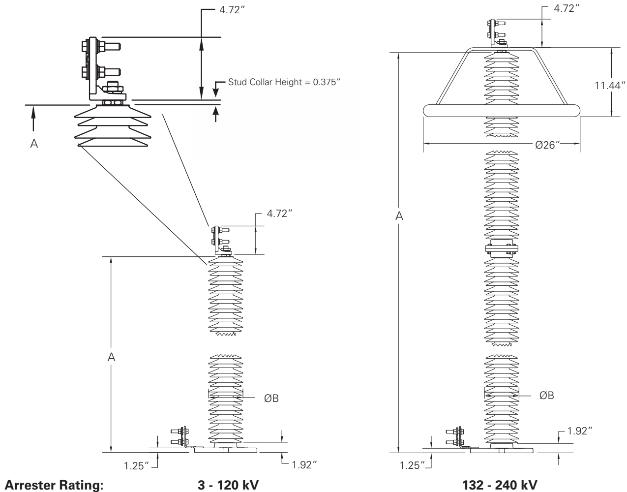
Figure 5. Outline drawing of standard UltraSIL Polymer-Housed Station-Class Arresters (for standard catalog numbers see Table 9).
