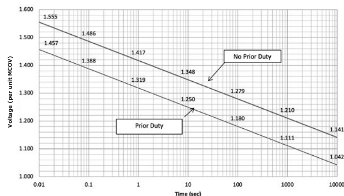
Figure 2. Temporary overvoltage curve – 60° ambient temperature.
