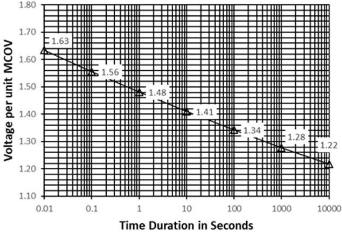
Figure 2. Temporary overvoltage curve. No prior duty at 85 °C.
