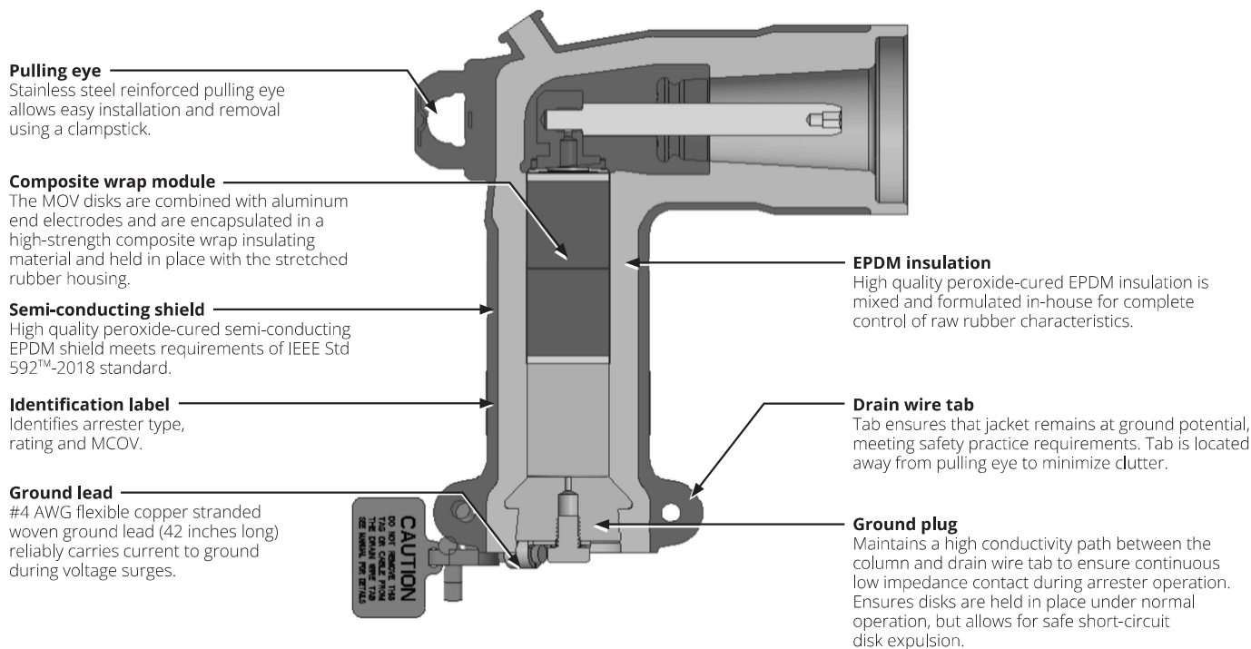
Figure 1. Cutaway illustration of deadfront elbow arrester.
