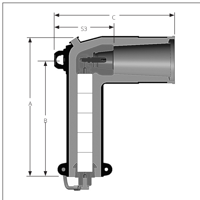
Figure 3. Dimensional information of DirectConnect elbow arrester
