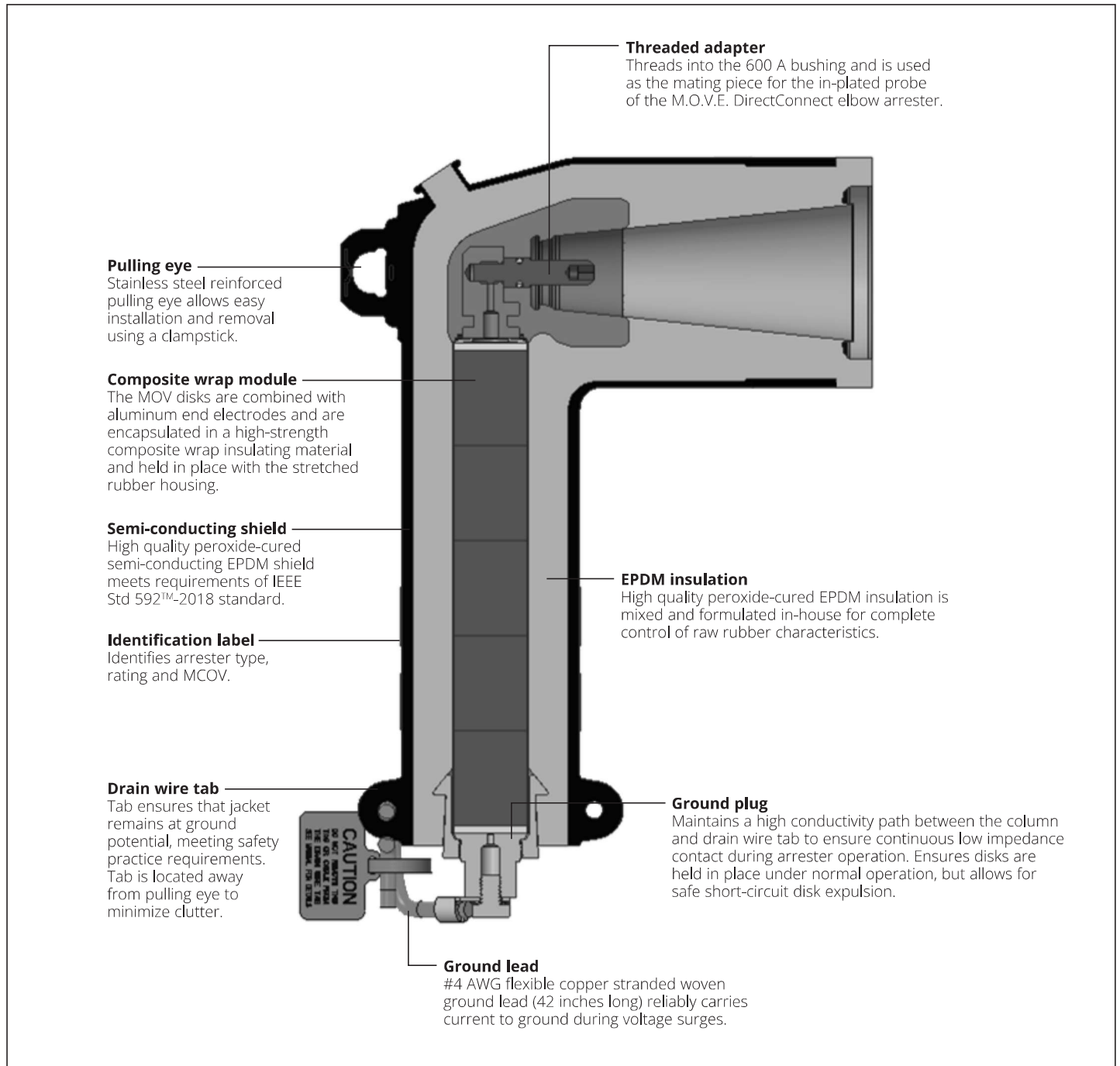
Figure 1. Cutaway illustration of DirectConnect deadfront elbow arrester
