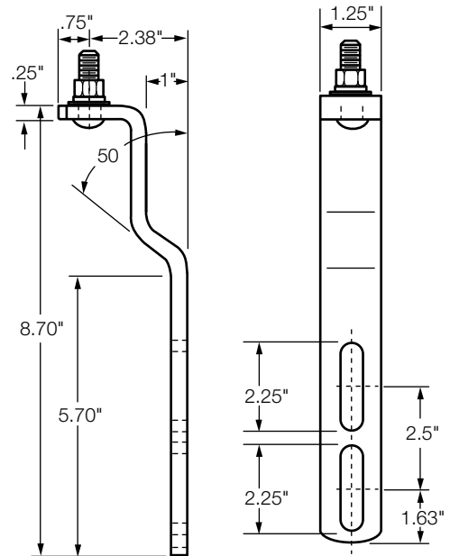
Figure 12. Standard transformer mounting bracket for 3-24 kV arrester (catalog number AM36A2) can be specified with a "C" in Digit 13 (all dimensions in inches)
