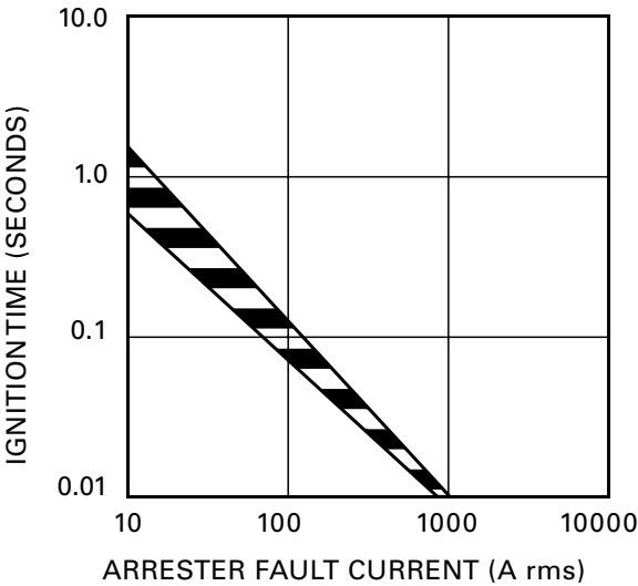
Figure 2. Isolator operating characteristic
