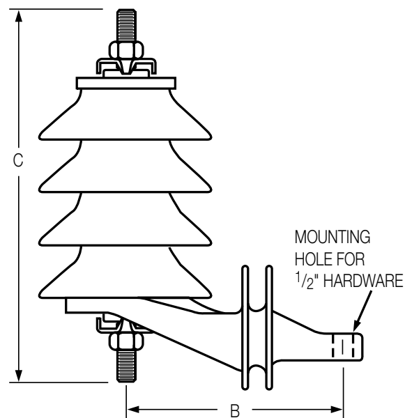
Figure 6. Evolution surge arrester without isolator including insulated hanger and NEMA cross-arm bracket
