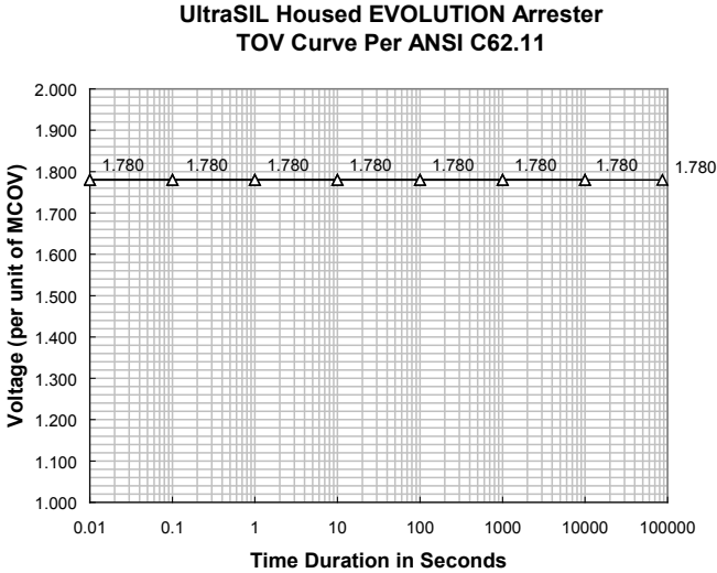
Figure 7. Temporary overvoltage curve, no prior duty—60 °C ambient
